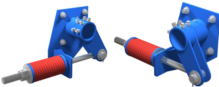
Mechanical Tensioner — CSHSMDST-01-N/A-A
