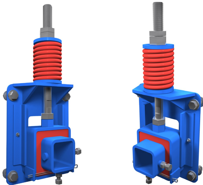
Pull-Up Mechanical Tensioner
